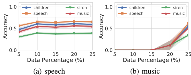
Fig. 9: Lowest amount of training data for speech (TIMIT+GAN-TIMIT) and music (Street Music). Shaded area around the lines represent the uncertainty. Speech is more robust for lower volume of training data.
