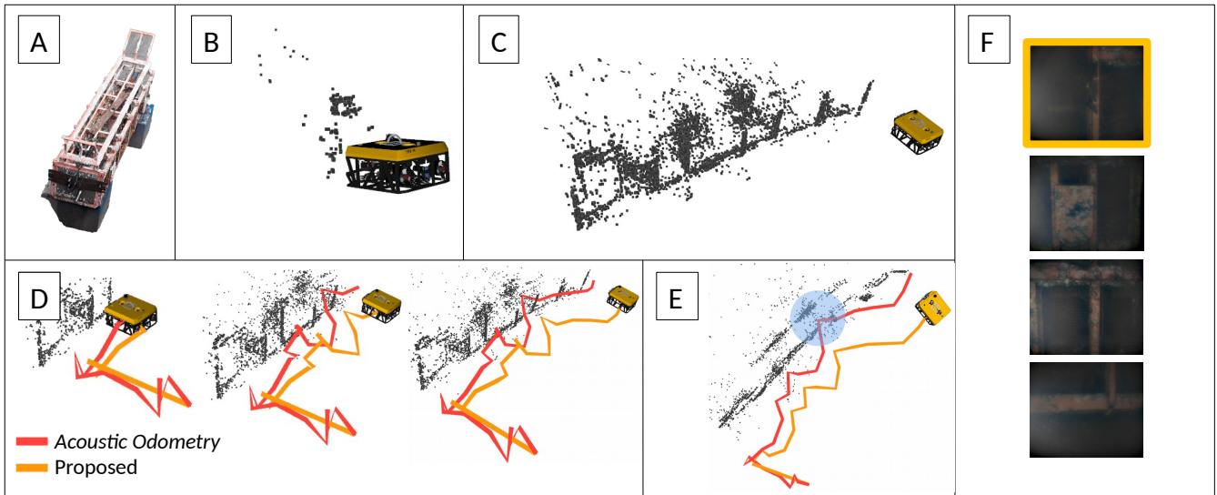
Fig. 6: In challenging visibility conditions, as the ones observed in BLYTH, the proposed approach outperforms ORB-SLAM2. [A] illustrates the submerged structure that was used for inspection. [B] is the result obtained with ORB-SLAM2, which loses track seconds after starting the inspection. [C] presents the obtained sparse reconstruction using the proposed approach. [D] shows snapshots of the trajectory estimated using our proposed approach (orange) and the one generated by acoustic odometry (red). [E] shows that the drift in acoustic odometry leads to an estimate which collides with the reconstruction (blue), while our method corrects for this drift using vision. [F] shows samples of images from this sequence. The image with the orange rectangle is the one in which ORB-SLAM2 loses track.
