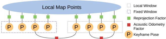
Fig. 2: Local BA factor graph. We introduce pair-wise pose constraints using acoustic odometry . The poses within the fixed window are not optimised but act as anchors for the pose constraints and the poses in the local window.
