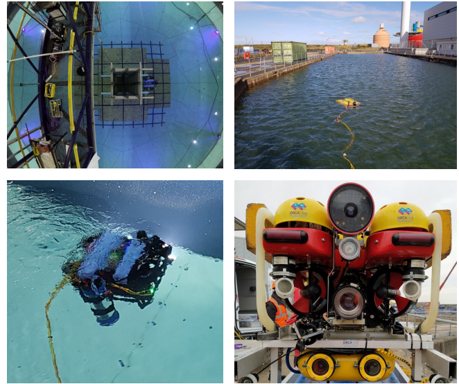
Fig. 1: Experiments were performed using BlueROV (bottom-left) and Falcon ROV (bottom-right). Both robots are equipped with a DVL, a gyroscope, an altimeter (Falcon ROV) / depth sensor (BlueROV) and a stereo camera. BlueROV was used in controlled conditions in an indoor tank (top-left) that contained an underwater motion capture system providing ground truth trajectory estimates. Falcon ROV was used to collect data in an indoor tank (in uncontrolled conditions) as well as during field trials in Blyth, UK (top-right).
