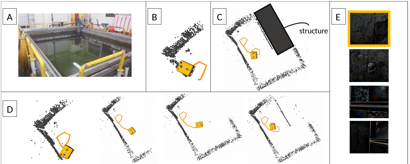
Fig. 4: The proposed algorithm reconstructs the walls of the tank in OSL-LOOP, while ORB-SLAM2 loses track after facing a feature-less area. [A] illustrates the OSL-tank, in which a structure was submerged. [B] is the result obtained with ORB-SLAM2, which loses track when facing one of the walls in the tank. [C] presents the obtained sparse reconstruction using the proposed approach. The area in which the structure was placed was highlighted in gray. [D] Illustrates snapshots of the trajectory and map estimated using our proposed approach, while [E] shows samples of images from this sequence. The image with the orange rectangle is the one in which ORB-SLAM loses track.
