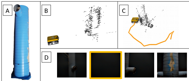
Fig. 7: In cases in which the robot loses view of the structure, the proposed approach outperforms ORB-SLAM2. [A] illustrates the submerged structure that was used for inspection. [B] is the result obtained with ORB-SLAM2, where the system loses track shortly after mapping began. [C] presents the obtained sparse reconstruction using the proposed approach, as well as the estimated trajectory. [D] shows the sequence of images. The image with the orange rectangle is the one in which ORB-SLAM2 loses track.
