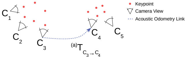
Fig. 3: If pose tracking is lost, we enable the system to initialise a new map as soon as we reach an area that can be tracked. We link the two maps using pose constraints from acoustic odometry .
